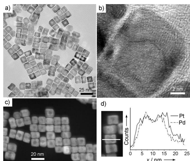
Figure 2. a, b) TEM images of Pd/Pt hollow nanocubes at low and high magnification; c) representative HAADF-STEM image of hollow nanocubes; d) line-scanning profile across a hollow Pd/Pt nanocube is indicated (left).
